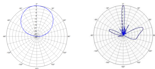
Horizontal Pattern
