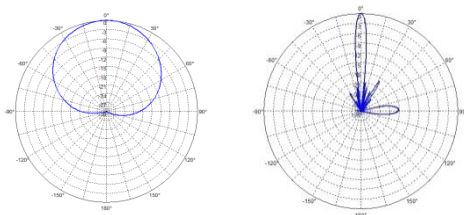
Horizontal Pattern
