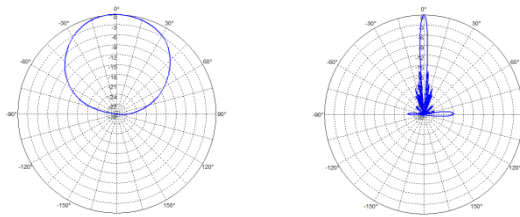
Radiation Patterns (3500-3800 MHz)
