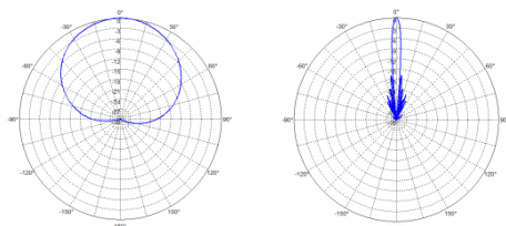
Radiation Patterns (3300 - 3500 MHz)
