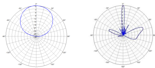
Radiation Patterns (3800-4200 MHz)
