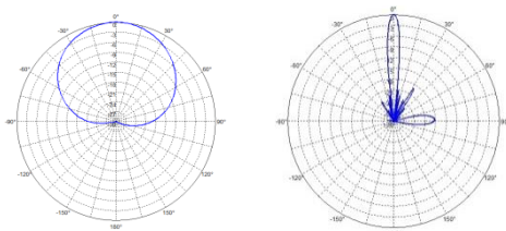
Radiation Patterns (3300 - 3800 MHz)
