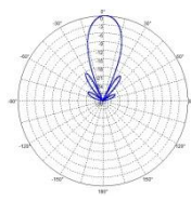
Vertical Pattern
