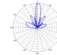
Vertical Pattern
