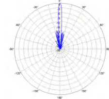
Vertical Pattern
