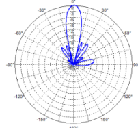
Vertical Pattern
