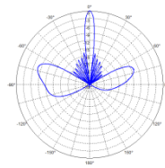
Vertical Pattern
