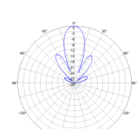
Radiation Pattern (2500- 2690 MHz)(Service Beam)
