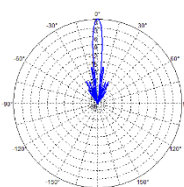
Radiation Pattern (2500- 2690 MHz)(Service Beam)
