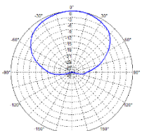
Radiation Pattern (2500- 2690 MHz)
