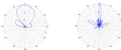
Horizontal Pattern
