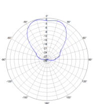
Horizontal Pattern
