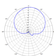
Horizontal Pattern
