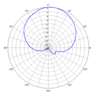
Horizontal Pattern
