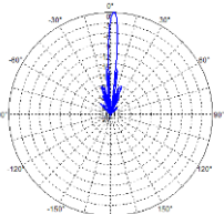
Vertical Pattern
